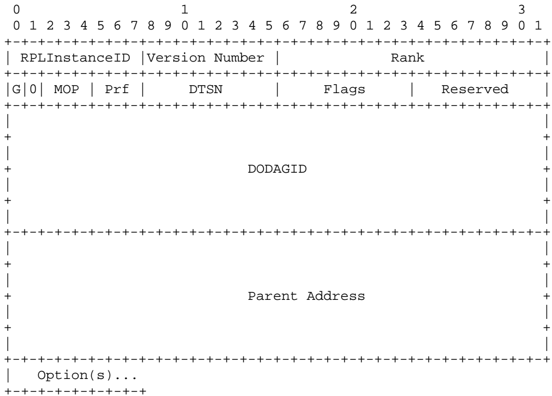
Figure 3: The amended DIO message format
